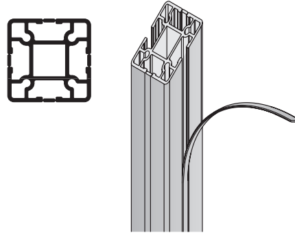
To release the channel, just pull off the protective aluminium strip
