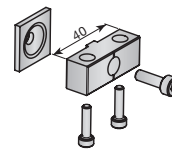
40mm joint to hold shelves at the corner.
