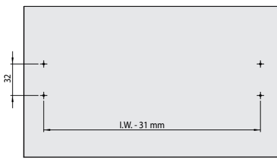
Drawer front
