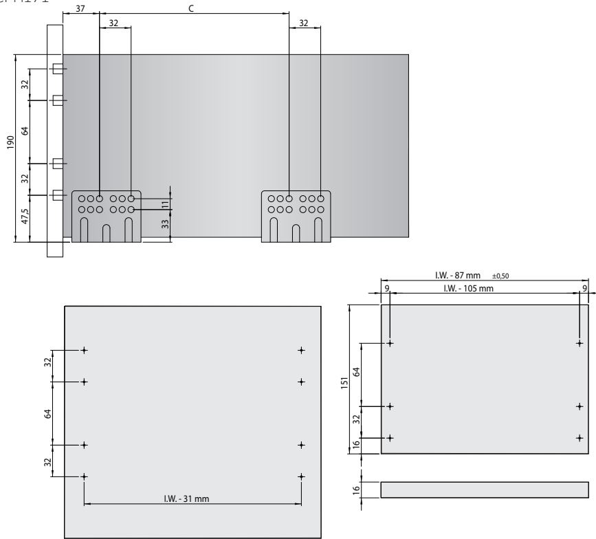
Drawer front
