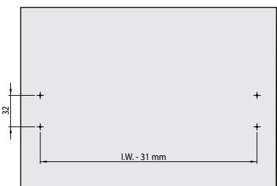
Drawer front
