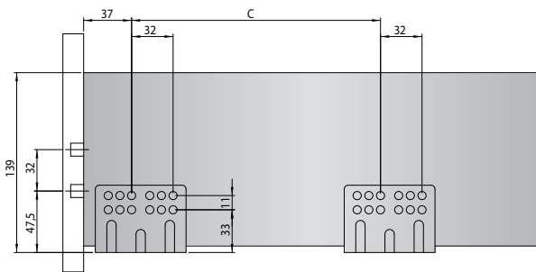
Drawer front
